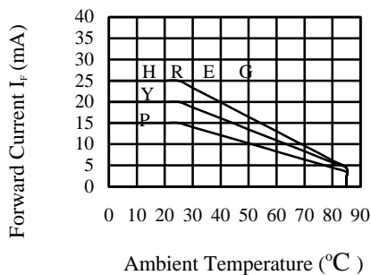
FIG.3 ALLOWABLE DC CURRENT VS. AMBIENT TEMPERATURE
